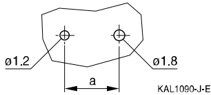
Suggestion for PCB hole diameter, wire ø1.0 mm
